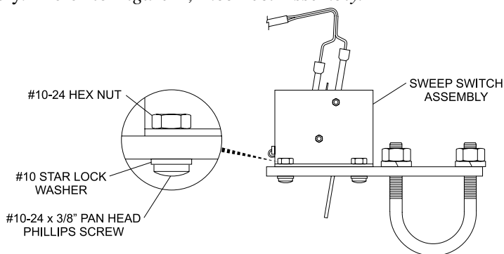
INCORRECT ASSEMBLY Figure 1
