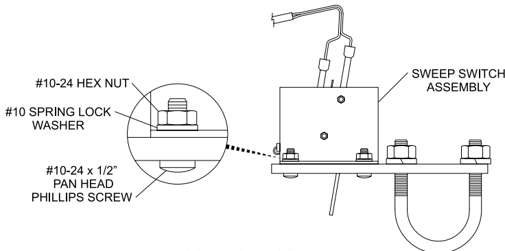
CORRECT ASSEMBLY Figure 2
