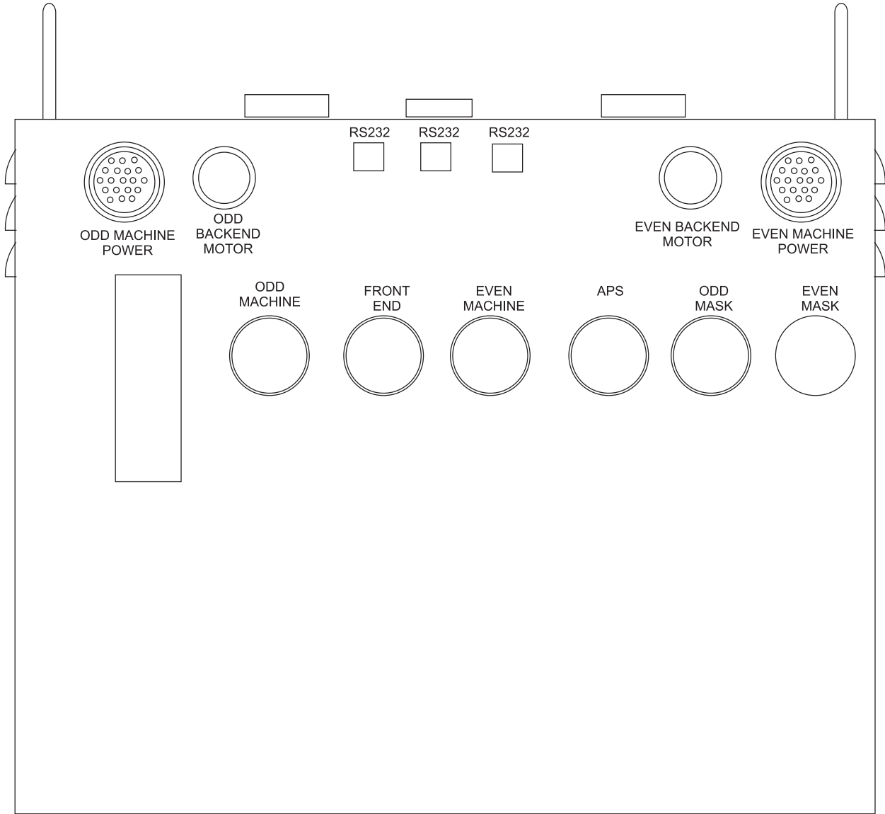
Figure 2 - Back of 8290XL Upgrade Chassis
