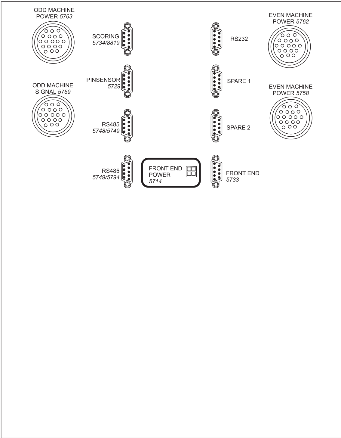
Figure 4 - Back of Silver Box 8290XL Chassis
