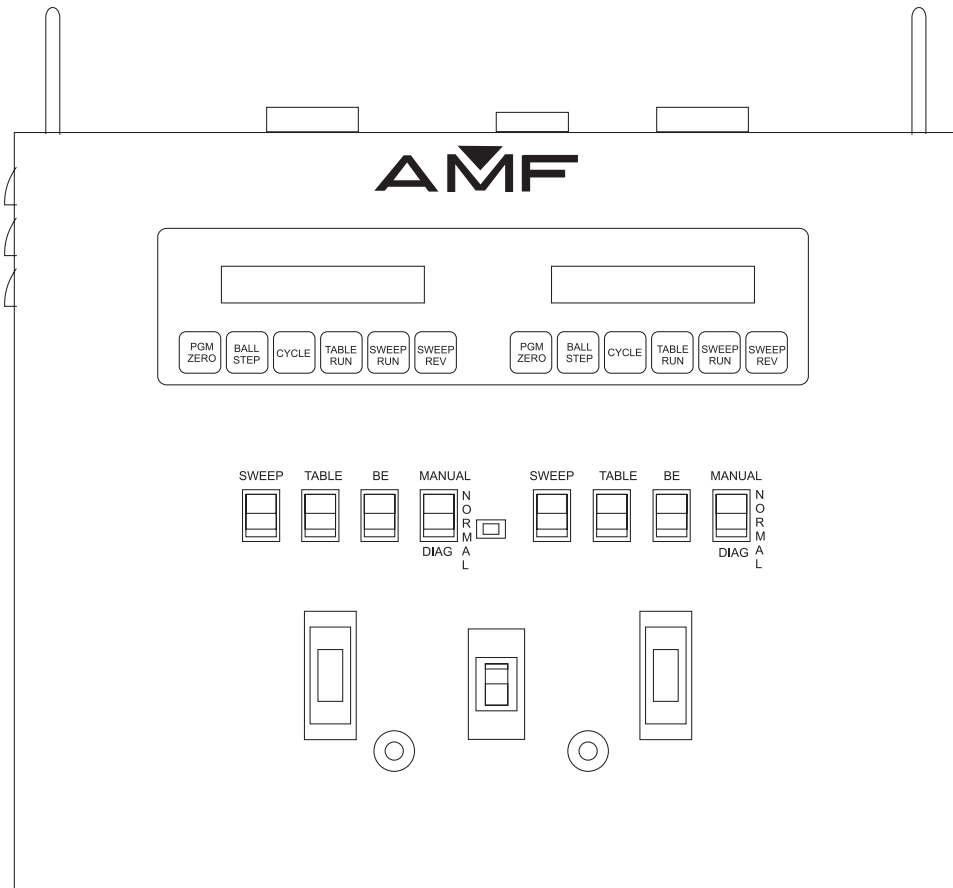
Figure 1 - Front of 8290XL Upgrade Chassis
