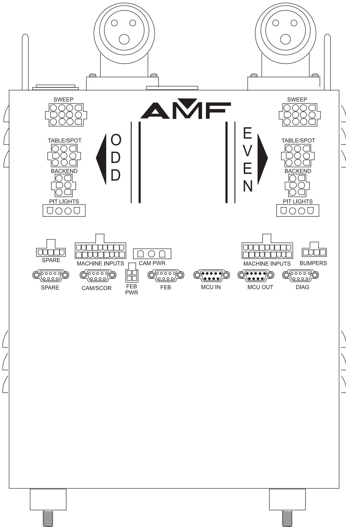
Figure 6 - Back of Black Box 8290XL Chassis
