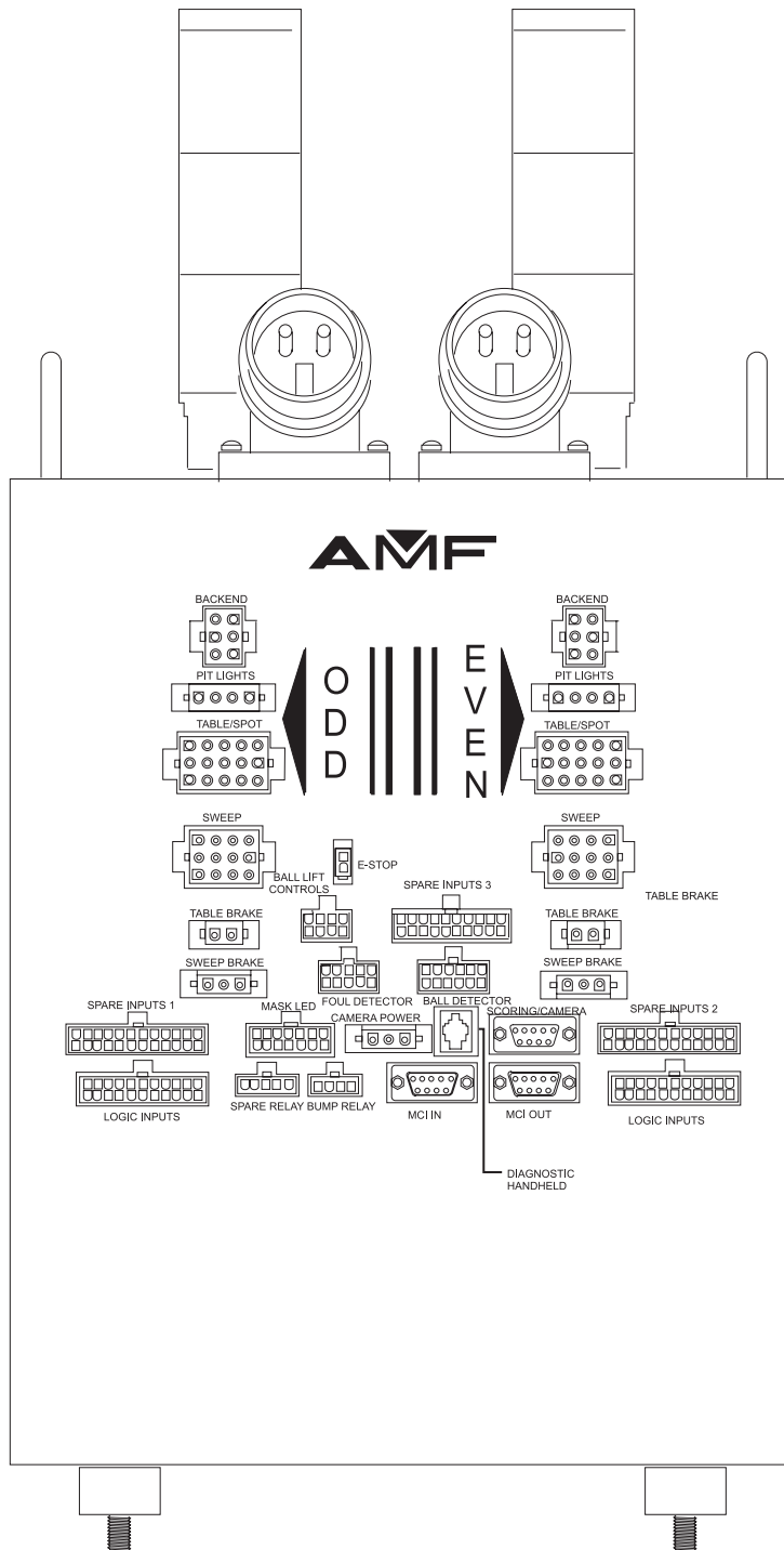
Figure 8 - Back of 8290XLi Chassis
